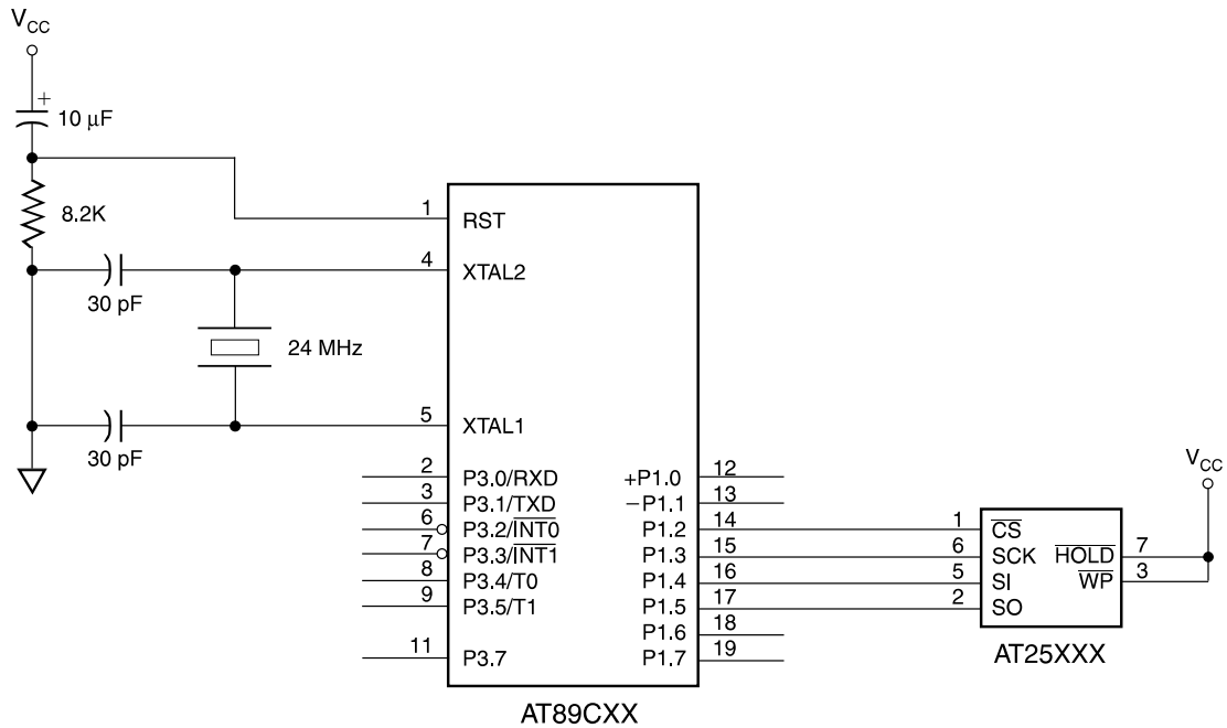
Figure 2. 4-Wire Configuration
