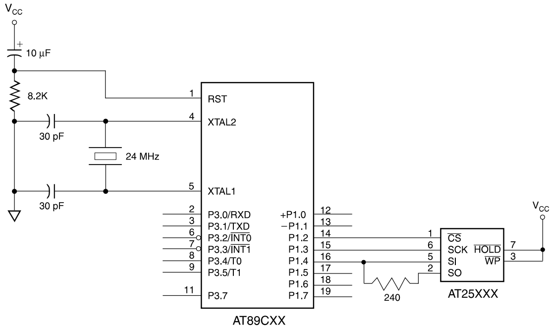
Figure 1. 3-Wire Configuration
